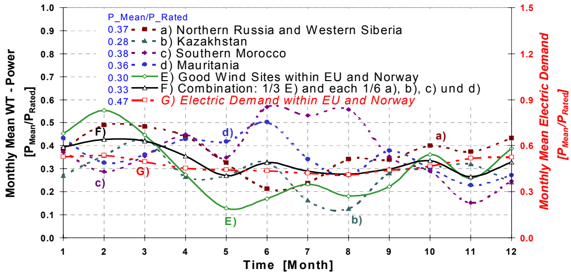
Figure 5 Relative monthly average: electricity production from wind turbines (WT) in selected good wind areas and electricity consumption of EU and Norway. a.) to d.) represent Extraeuropean production E.) represents European production and F.) is the combined production of wind power at all regions whereas G.) represents the average consumption in the EU & Norway weighted with the today's rated power of all power plants installed.
