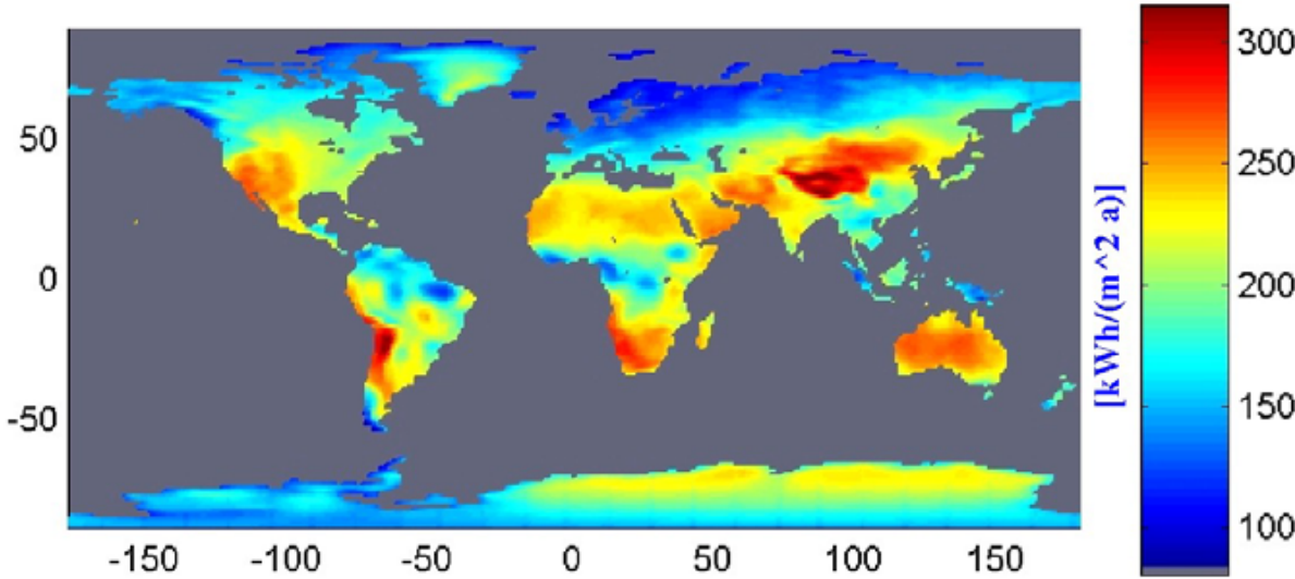
Figure 2 Potentials for average electricity production from photovoltaic generation derived for the years 1983-1992 Module = 14%, System = 11.5%, Orientation East-West with Slope = Latitude; met. data: ECMWF and NCEP.
